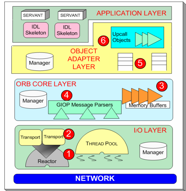
Figure 1. Layered CORBA Request Processing
