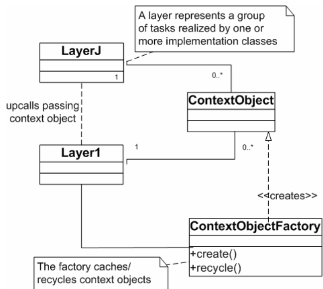
Figure 2. Structure of Context Object Pattern
