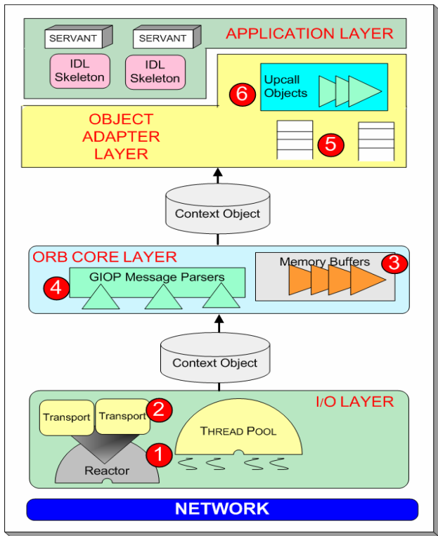
Figure 4: Layered CORBA demultiplexing using Context Object
